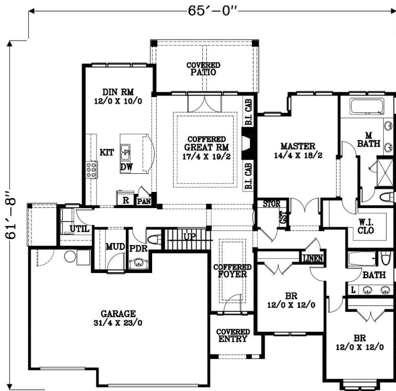
MAIN FLOOR 2230 SQUARE FEET 2558 SQUARE FEET TOTAL
