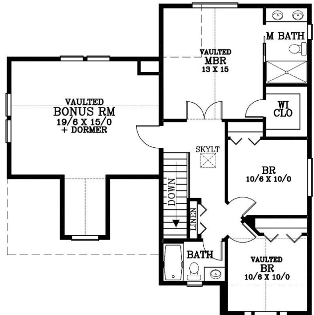
UPPER FLOOR PLAN 744 SQUARE FEET NIC 352 S.Q. FT. BONUS RM
