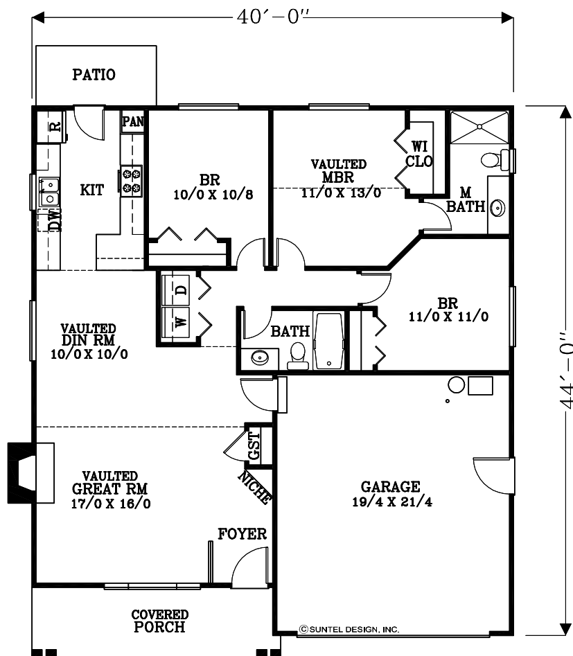
FLOOR PLAN 1252 SQUARE FEET
