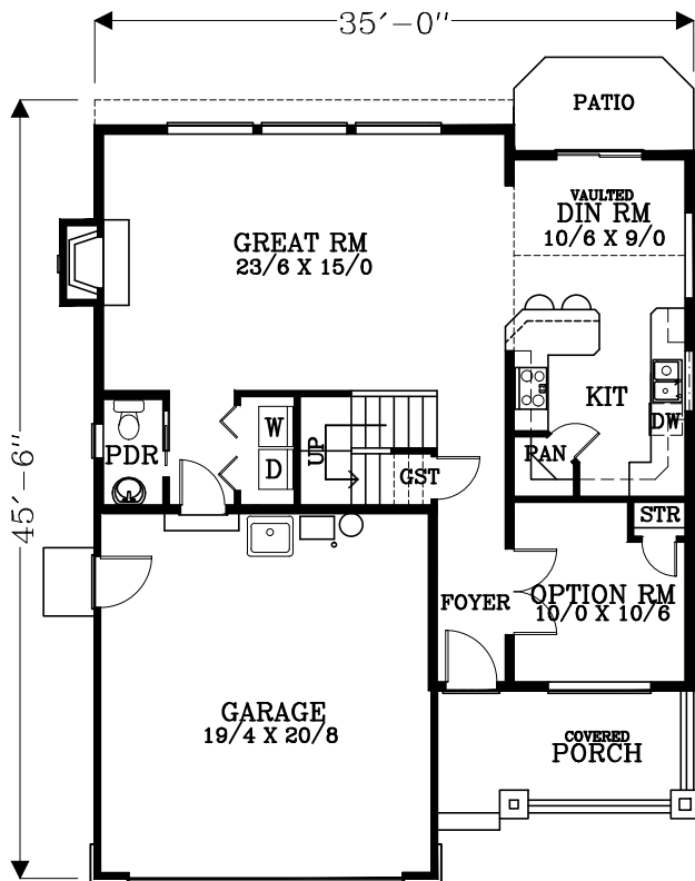
MAIN FLOOR PLAN 920 SQUARE FEET 1780 TOTAL SQUARE FEET
