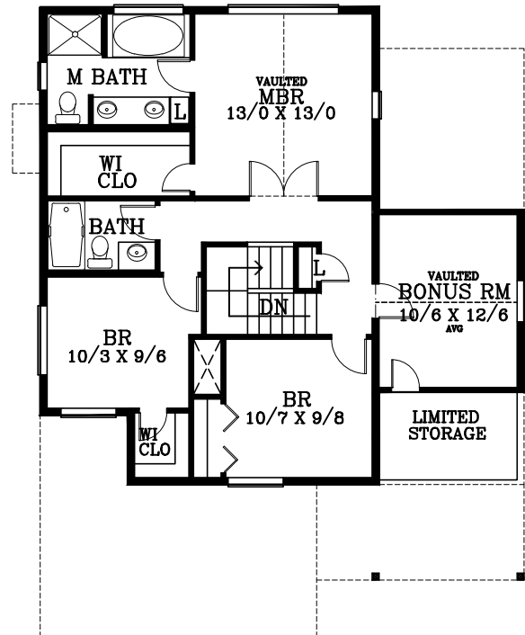
UPPER FLOOR PLAN 860 SQUARE FEET
