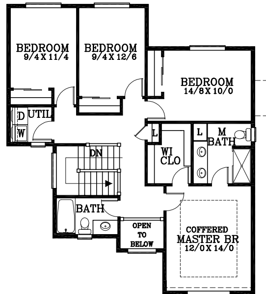
UPPER FLOOR PLAN 991 SQUARE FEET
