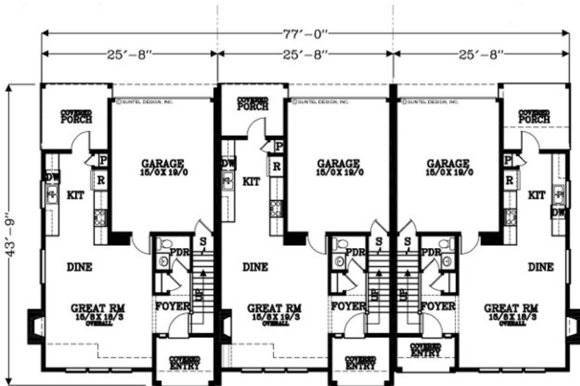
MAIN FLOOR PLAN 597 SQUARE FEET 1574 TOTAL SQUARE FEET
