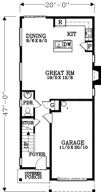
MAIN FLOOR PLAN 616 SQUARE FEET 1470 TOTAL SQUARE FEET
