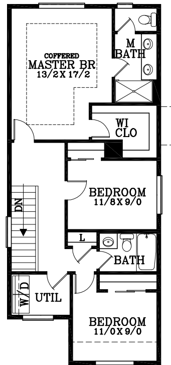
UPPER FLOOR PLAN 854 SQUARE FEET
