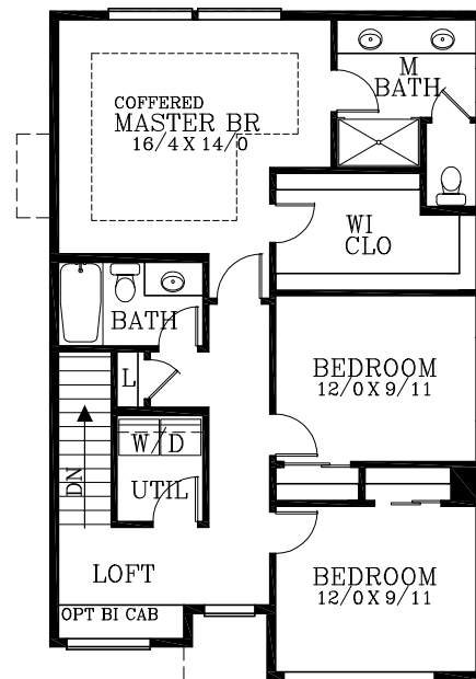
UPPER FLOOR PLAN 967 SQUARE FEET
