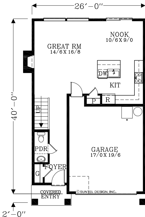
MAIN FLOOR PLAN 664 SQUARE FEET 1631 TOTAL SQUARE FEET
