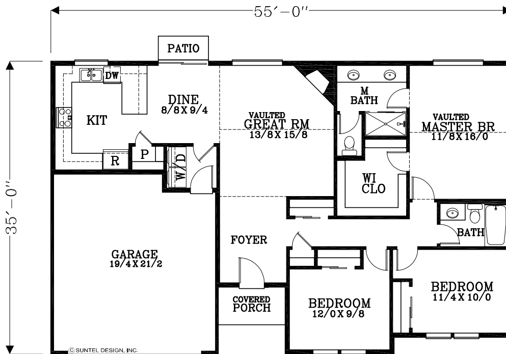
FLOOR PLAN 1,421 TOTAL SQUARE FEET
