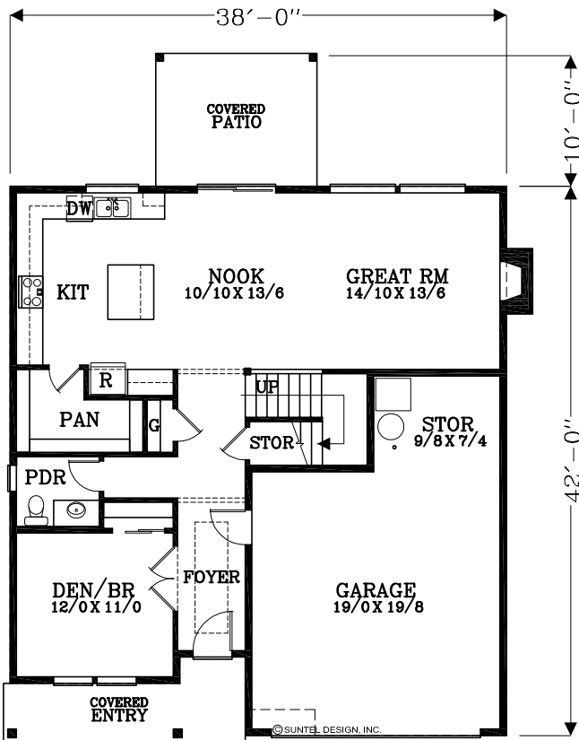
MAIN FLOOR PLAN 1,043 SQUARE FEET 2,477 TOTAL SQUARE FEET
