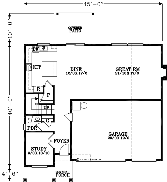
MAIN FLOOR PLAN 1,120 SQUARE FEET 2,383 TOTAL SQUARE FEET
